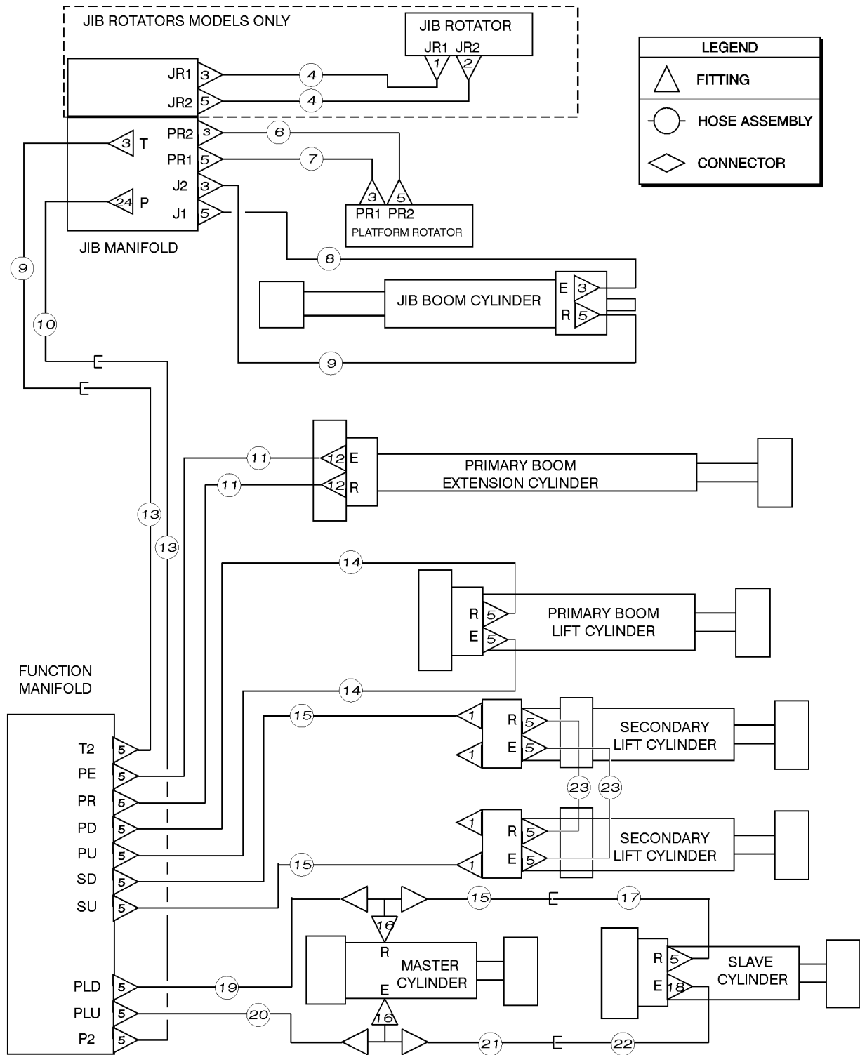
Z40 703.1 Boom Components
